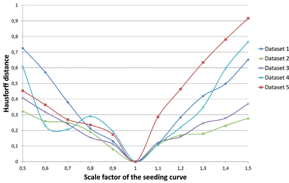
Fig. 8. Robustness in terms of the seeding contour variation and the Hausdorff distances between resulting boundary contours.
