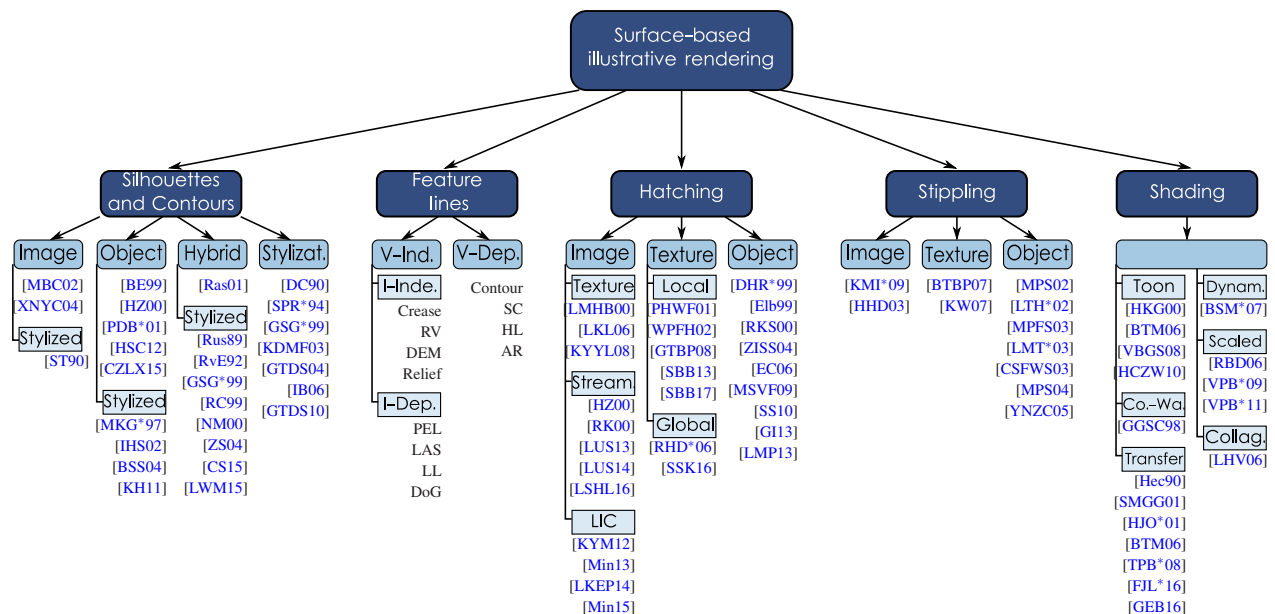
Figure 10: An overview of the discussed illustrative visualization techniques. Every field is divided into different categories, which reflects the sub-sections of the corresponding section. Note that the lists of specific papers for each approach only serve as examples.
