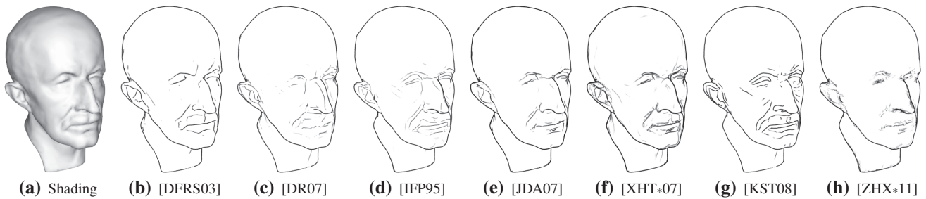
Figure 4: This overview shows the different feature line techniques applied to the Max Planck model. From left to right: shading, suggestive contours, suggestive highlights, ridges and valley, apparent ridges, photic extremum lines, demarcating curves and Laplacian lines.
